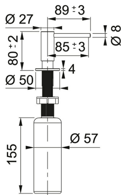
Technical Drawing
